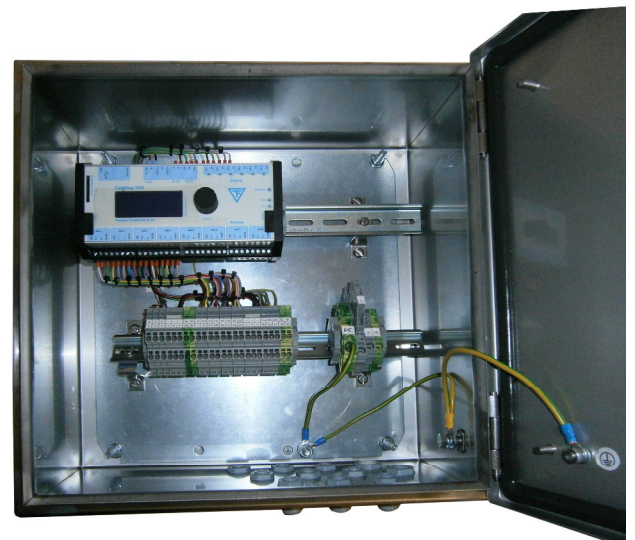
COMBILOG 1022, built in Stainless Steel Housing Type 9930.1000
